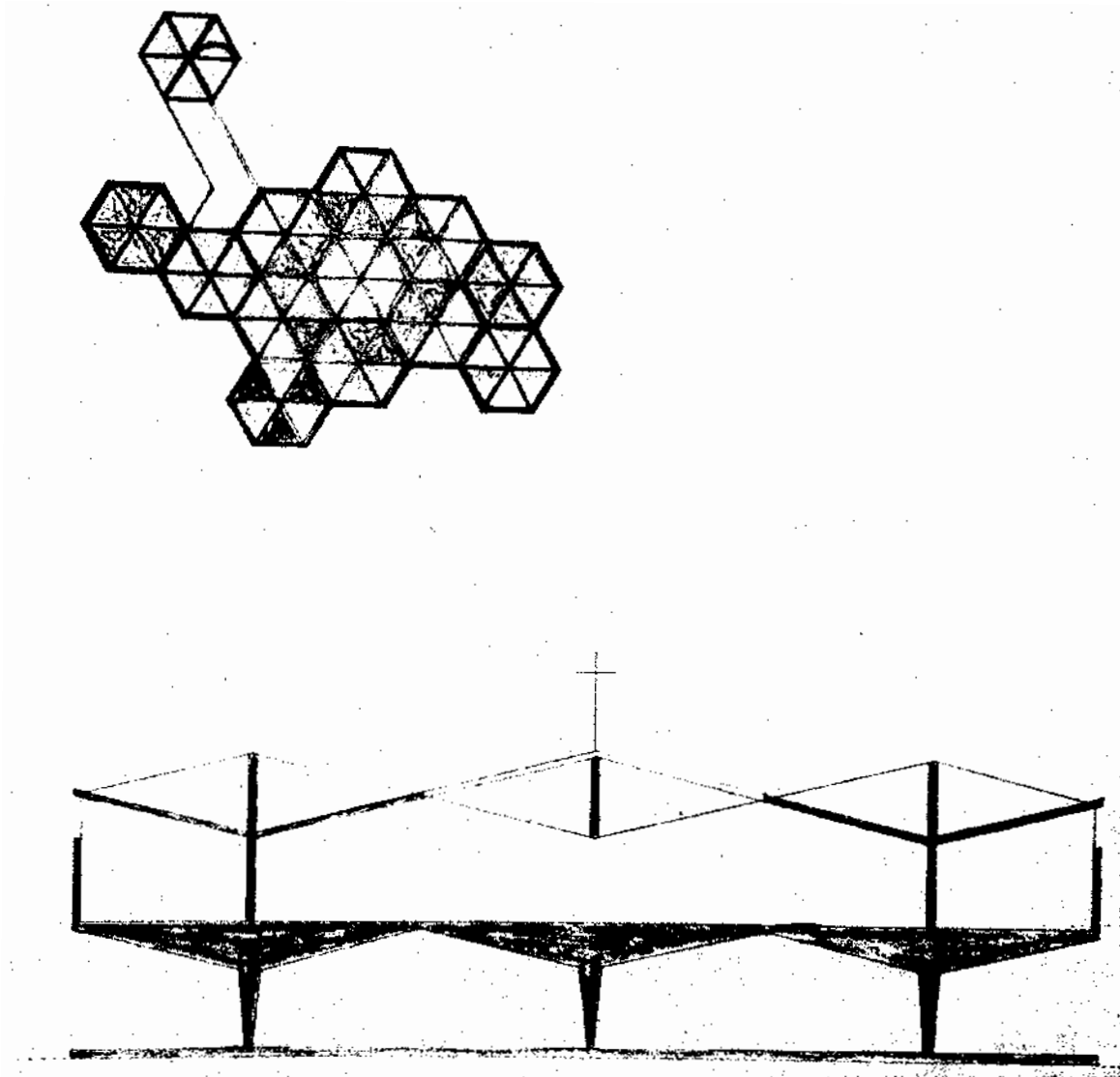
Tony Smith's plan for a Catholic church. 1950-51. The upper portion represents the church's ceiling, the lower, a central cross-section.
